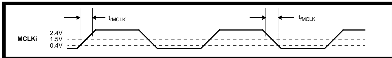
Figure 7 - Master Clock Input
